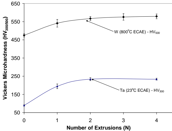
Fig. 3. Vickers microhardness as a function of the number of extrusion passes for Ta and W. The error bars indicate the standard deviation of the measurements.
