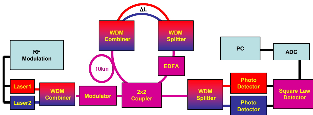
Figure 2 Simplified diagram of channelizer demonstration experimental set-up
